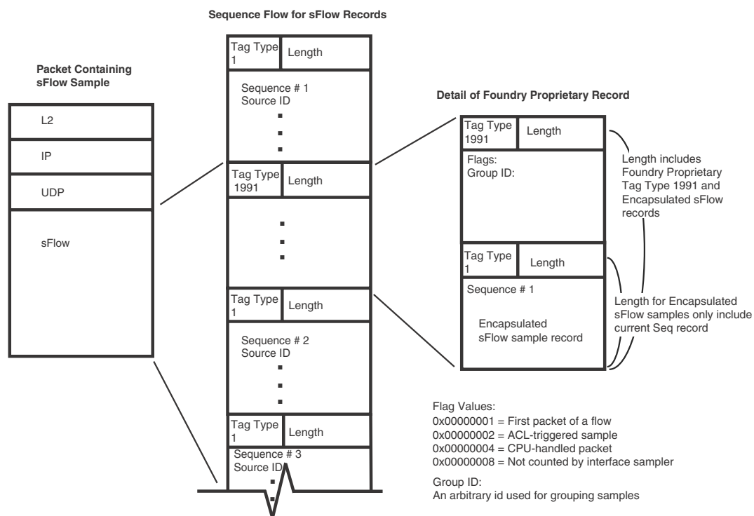
FIGURE 138 sFlow packet format
